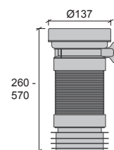
A WC - Stos, X-tra Flexibel RSK 310 67 28
